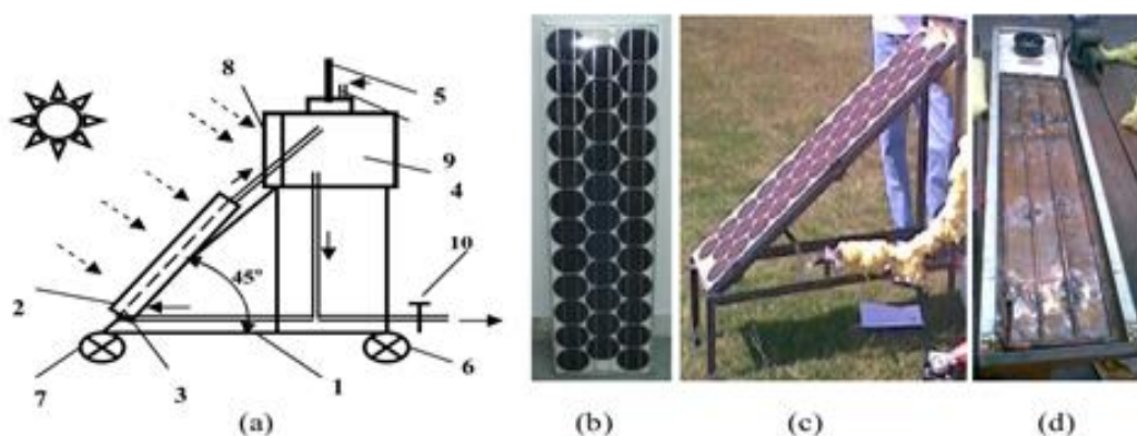
Photo 2. A hybrid solar system of the “photovoltaic module-collector” type.
